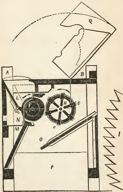
COTTON GIN.
